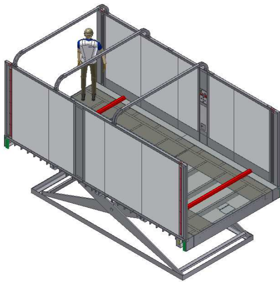
CAD 3D-design
